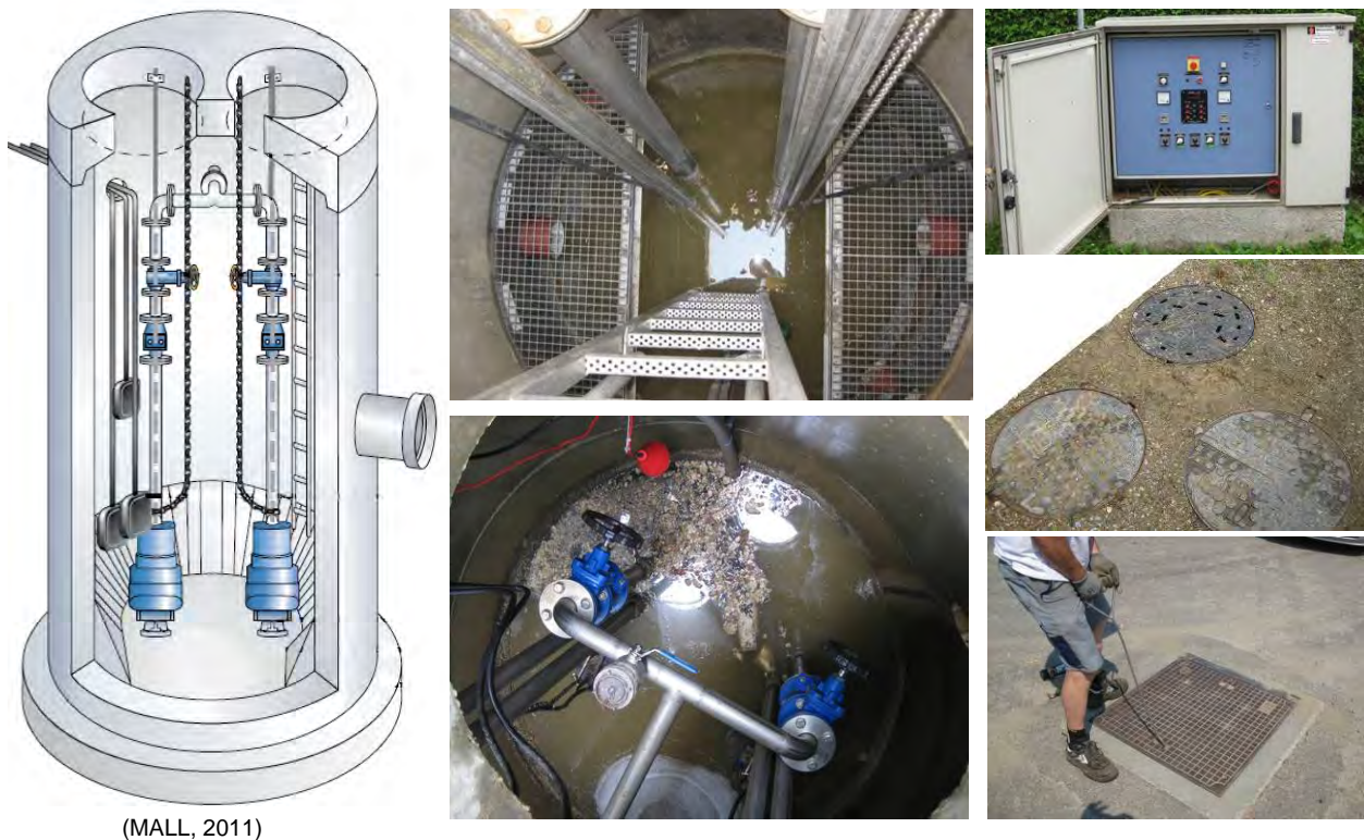
Abbildung 8-5: Standardpumpstation
